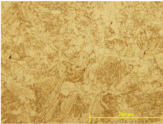
Figure 5. Microstructure of the LM sample tempered at 700 °C
