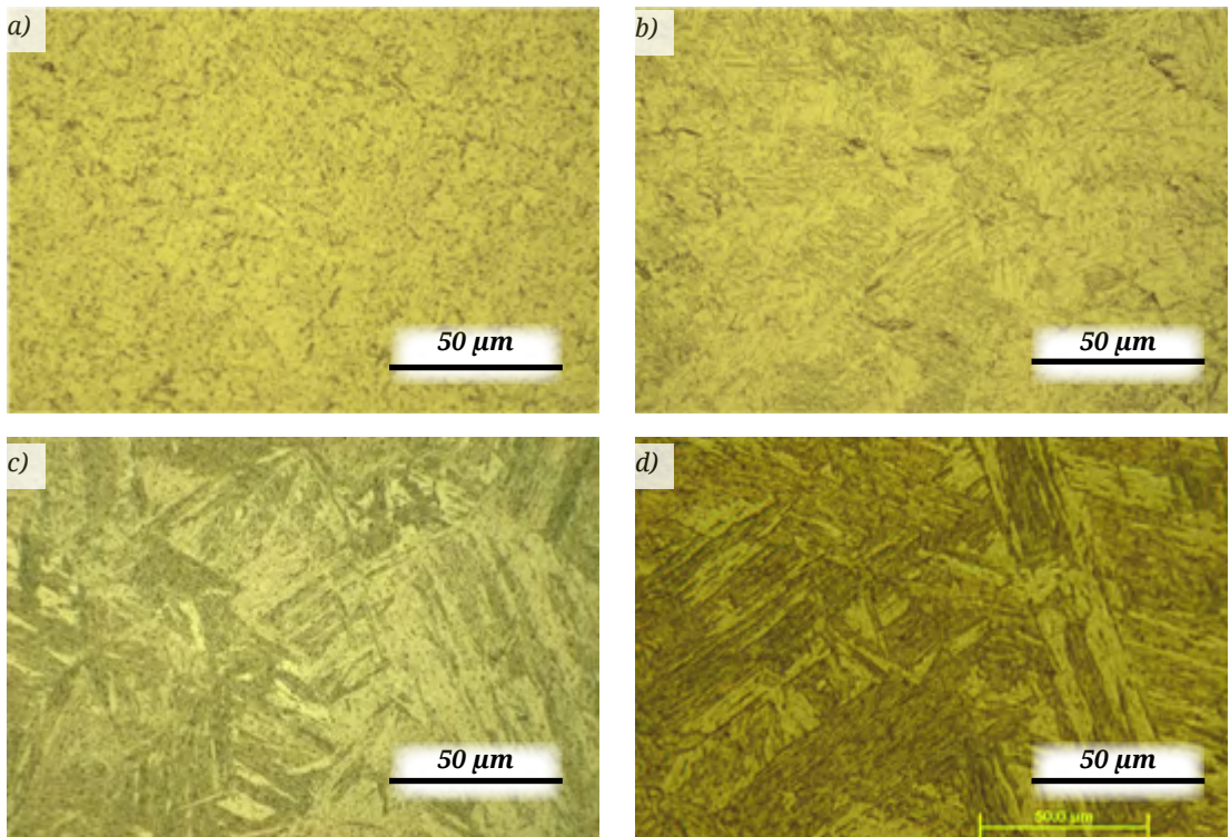
Figure 1. The effects of austenitization temperatures on the microstructure a) T_{aust} = 900\text{ °C} ; b) T_{aust} = 1000\text{ °C} ; c) T_{aust} = 1100\text{ °C} d) T_{aust} = 1200\text{ °C}
