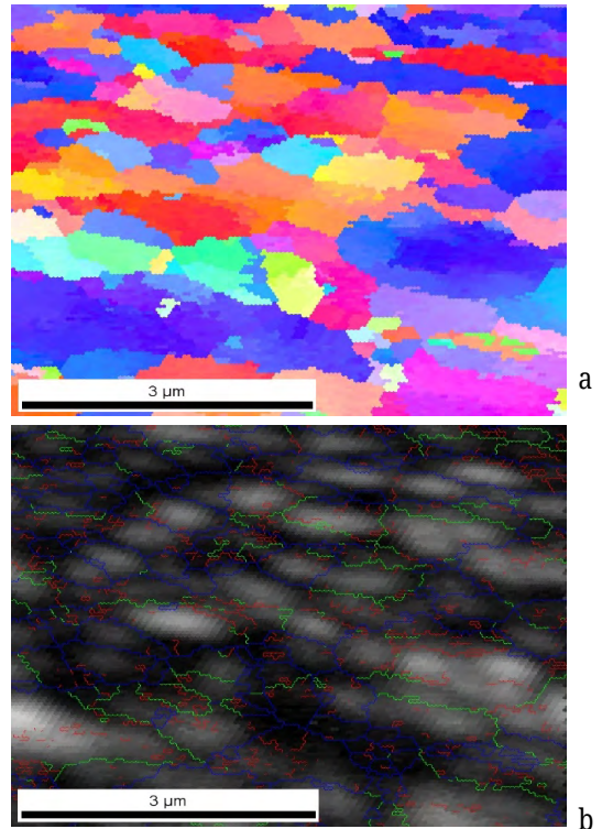
Figure 8. EBSD images, \epsilon=44\% , T=500^\circ\text{C} , N=10000x . a) Pole figure map b) Image quality map
