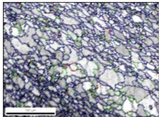
Figure 9. Image quality map at sample, 86%, T=700^\circ\text{C}
